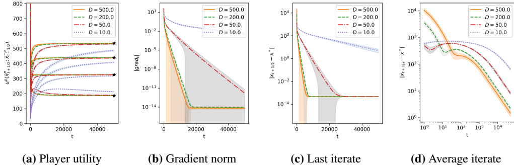
Figure H.5: We compare the effect of the diameter choice for adaptive DualX on a Kelly auction with \sigma_{\text{rel}} = 0.2 . We can observe the \mathcal{O}(1/T) average iterate rate for the whole spectrum of diameters but we note that the choice of diameter still has practical impact on convergence time. The fastest convergence is achieved with the highest diameter but note that the method did not converge for D = 1000 which we have excluded to keep the plots readable.
