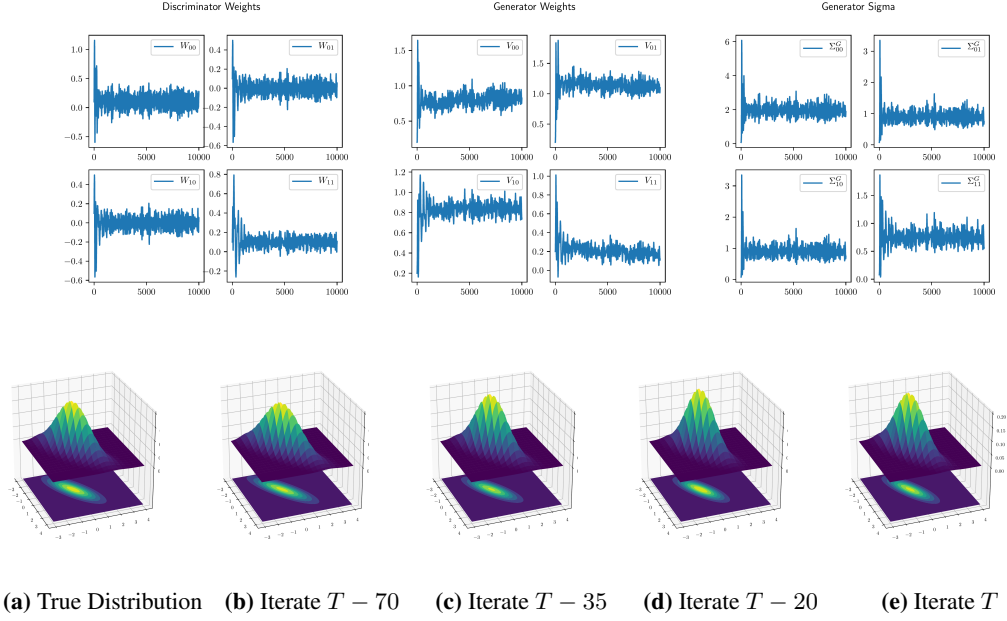
Figure H.8: OG for covariance learning of a two-dimensional gaussian without weight clipping using a batch size of 50. Comparison of true distribution and distribution of generator at various points at the end of training.
