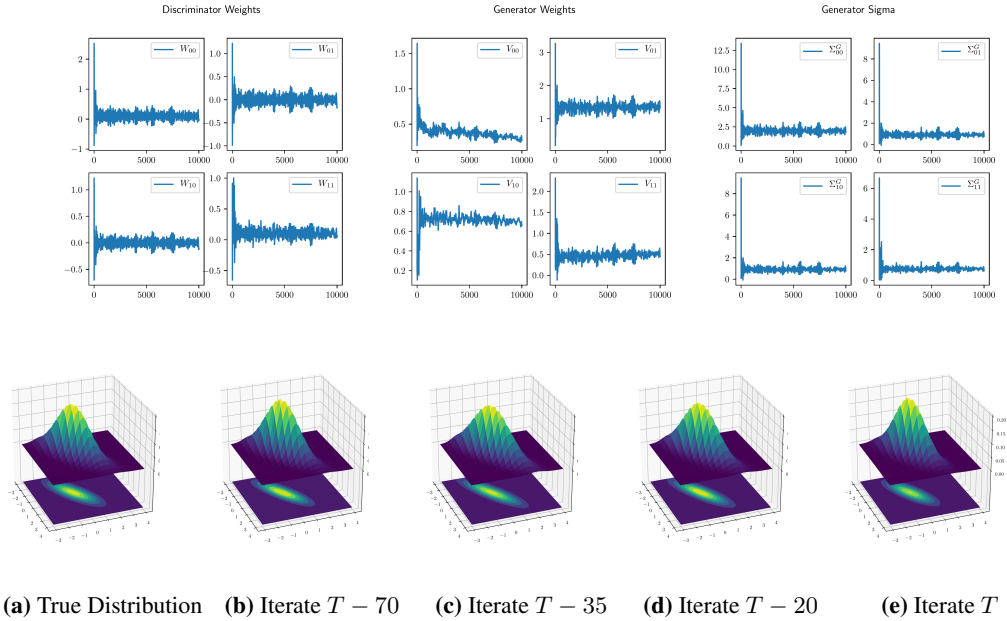
Figure H.9: Adaptive DualX for covariance learning of a two-dimensional gaussian without weight clipping using a batch size of 50. Comparison of true distribution and distribution of generator at various points at the end of training.
