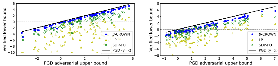
(a) MNIST CNN-A-Adv, runner-up targets, ε = 0.3
