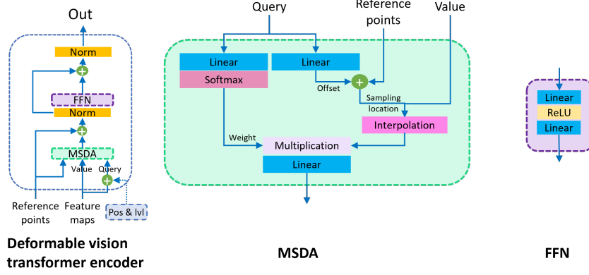
Figure 2: Left: The structure of the deformable vision transformer encoder. It is the same as the encoder in DETR except that the key tensor is removed while reference points are required. Mid: The MSDA averages the features at sparse sampling locations across different scales with weights computed from the query tensor. Right: Feed-Forward Network (FFN).
