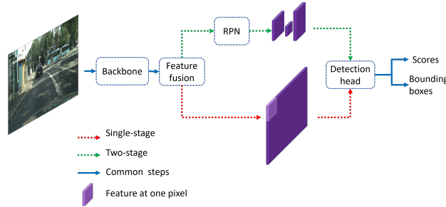
Figure 1: Generic detection pipeline of the single- and two-stage detectors. The detection head consists of two parallel branches for classification and regression.
