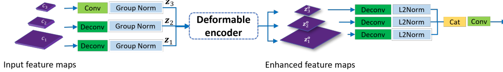
Figure 3: The overall architecture of the proposed feature enhancement module.
