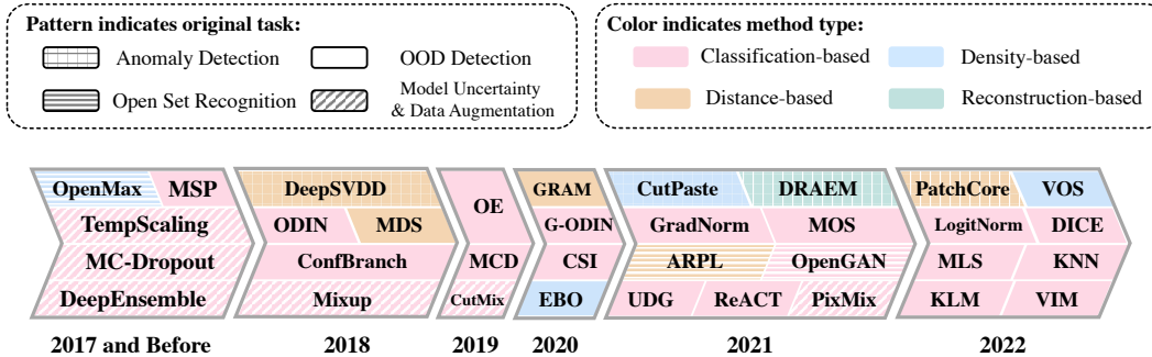
Figure 2: Timeline and Taxonomy of Methodologies supported by OpenOOD. OpenOOD supports 35 methods (by the time of publication) that originated from anomaly detection (AD), open set recognition (OSR), OOD detection, and model uncertainty & data augmentation. Methodologies can be categorized into classification-based, density-based, distance-based, and reconstruction-based ones.
