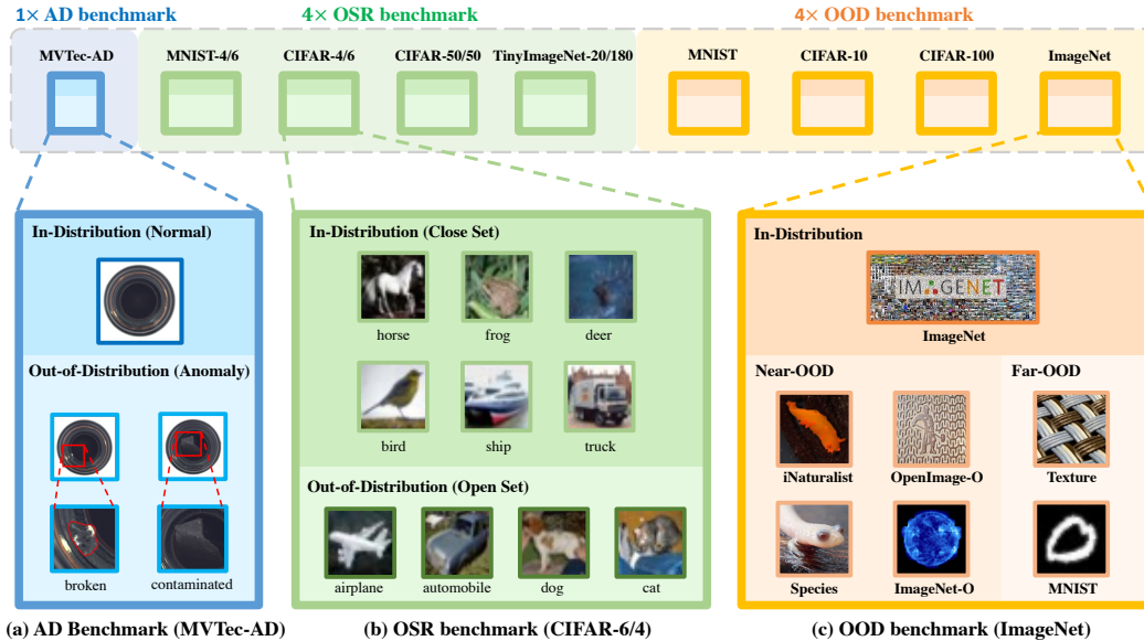
Figure 1: Diagram of benchmarks supported by OpenOOD. OpenOOD supports 9 benchmarks that originated from anomaly detection (AD), open set recognition (OSR), and OOD detection. Three example benchmarks are highlighted to represent AD, OSR, and OOD detection, respectively. The different benchmarking styles of AD, OSR and OOD detection clearly indicate their focus. While AD requires models to be aware of the pixel-level difference like scratch, OSR and OOD detection focuses on detecting the semantic shift, where OOD (open-set) samples come from other dataset (other label-split of the dataset). All those benchmarks can be easily downloaded via this script .
