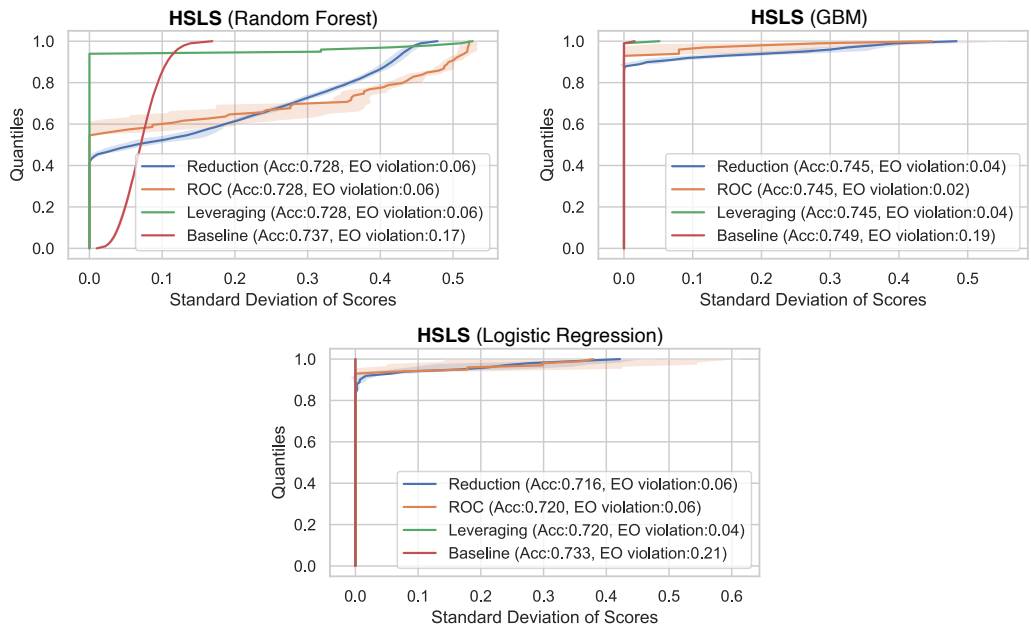
Figure 17: Quantile plot on models in high-fairness bin for various fairness interventions v.s. baseline models on HSL. Fair models produce larger score std. at top percentiles compared to the baseline model.
