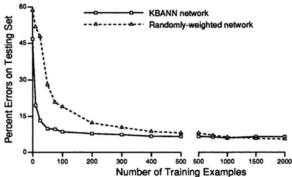
Figure 4: Learning Curve for Splice Junctions
