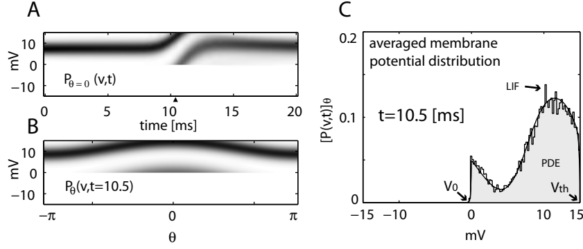
Figure 2: A: Dynamics of membrane potential distribution at \theta = 0 . B: A snapshot of the membrane potential distributions for a range of [-\pi \pi] at t = 10.5 . C: A snapshot of the membrane potential averaged with position \theta . Results by a numerical simulation (LIF) and the Fokker-Planck equation (PDE) are shown.
