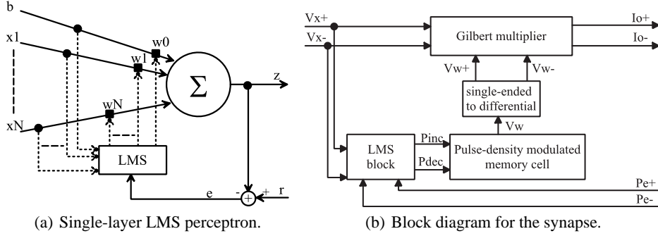
Figure 1: A single-layer perceptron and synapse. (a) The output z of the perceptron is the inner product between the input and weight vectors. The LMS algorithm updates the weights based on the inputs and an error signal e . (b) The synapse stores the weight in an analog memory cell. A Gilbert multiplier computes the product between the input and the weight and outputs a differential current. The LMS block updates the weight.
