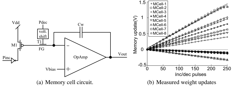
Figure 3: A simple PDM analog memory cell. (a) We store each weight as nonvolatile analog charge on the floating gate FG. The weight increments and decrements are proportional to the density of the pulses on P_{inc} and P_{dec} . (b) Memory updates as a function of the increment and decrement pulse densities for 8 synapses. The updates show excellent linearity (10 bits), but also poor matching both within a synapse and between synapses.
