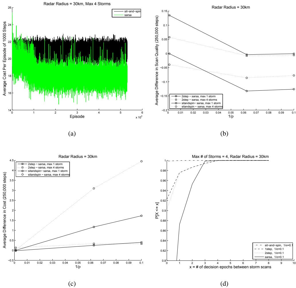
Figure 2: Comparing the scan strategies based on quality, cost, and inter-scan time. Recall that \rho is a scaling term used to determine measurement noise, see Section 4.1.
