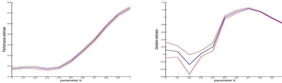
Figure 2: Left: Estimator \frac{1}{M} \sum_{m=1}^M J_{\omega_m}^N(\theta) of J(\theta) and confidence intervals \pm \sqrt{\text{Var}[J_{\omega}^N(\theta)]/M} . Right: Estimator \frac{1}{M} \sum_{m=1}^M \partial_h J_{\omega_m}^N(\theta) of \partial J(\theta) and confidence intervals \pm \sqrt{\text{Var}[\partial_h J_{\omega}^N(\theta)]/M} .
