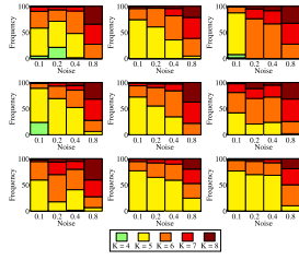
Figure 1: The posterior distribution of K .
