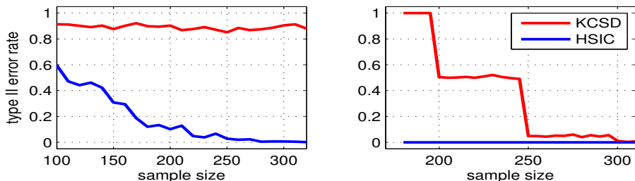
Figure 2: In both panel Type II error is plotted. The left panel presents the error of the lag-HSIC and KCSD algorithms for a process following dynamics given by the equation (6). The errors for a process with dynamics given by equations (7) and (8) are shown in the right panel. The X axis is indexed by the time series length, i.e., sample size. The Type I error was around 5%.
