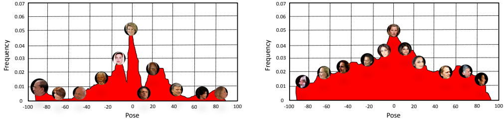
(a) Extremely unbalanced pose distribution. (b) Well balanced pose distribution with DA-GAN.
