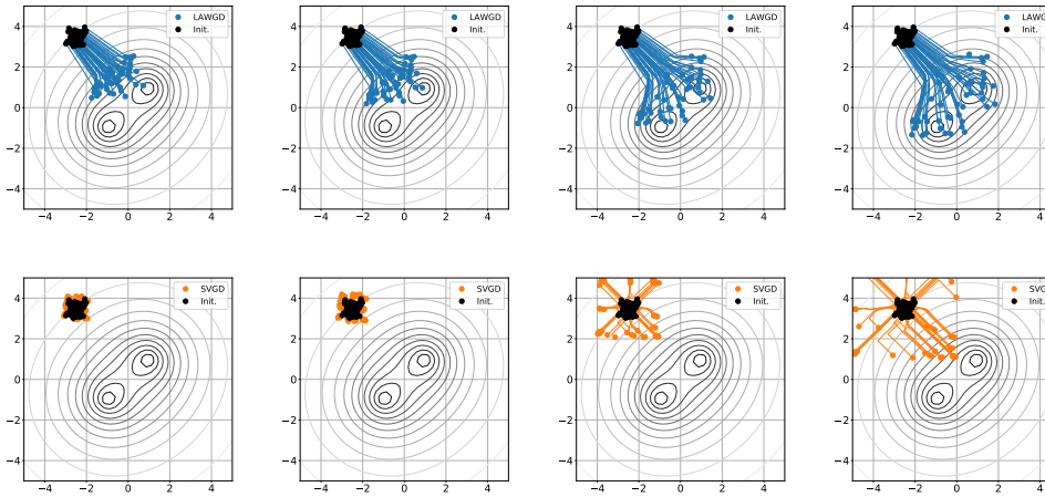
Figure 5: Top: LAWGD after 100, 200, 1000, and 2000 iterations. Bottom: SVGD after 100, 200, 1000, and 2000 iterations.
