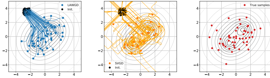
Figure 4: Left: 50 particles and trajectories generated from \frac{1}{2}\mathcal{N}((-1, -1)^\top, I_2) + \frac{1}{2}\mathcal{N}((1, 1)^\top, I_2) with LAWGD . Middle: 50 particles and trajectories generated by SVGD . Right: true samples from the distribution.
