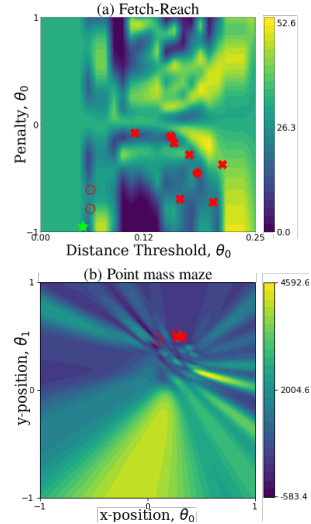
Figure 6: BO-IRL’s GP posteriors for (a) Fetch-Reach task environment and (b) Point Mass Maze.
