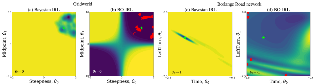
Figure 5: Posterior distribution over reward functions recovered by BIRL for (a) Gridworld environment and (c) Börlänge road network, respectively. The GP posteriors over NLL learned by BO-IRL for the same environments are shown in (b) and (d). The red crosses represent samples selected by BO that have NLL better than the expert’s true reward function. The red filled dots and red empty dots are samples whose NLL are similar to the expert’s NLL, i.e., less than 1% and 10% larger, respectively. The green \star indicates the expert’s true reward function.
