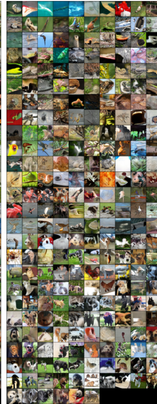
Figure 7: Rand-DP-OAdam
