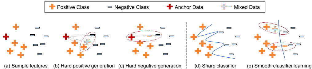
Figure 1: Illustration of two challenges in contrastive fine-tuning. (1) How to mine hard sample pairs for more effective contrastive fine-tuning. As shown in (a), the majority of sample pairs are easy-to-contrast, which may induce negligible contrastive loss gradients that contribute little to learning discriminative representations. (2) How to improve the generalizability of the model. As shown in (d), the classifier simply trained with cross-entropy is often sharp and near training data, leading to limited generalization performance.
