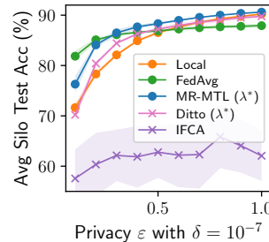
Figure 4: The privacy overhead of cluster selection (IFCA) and extra iterations (Ditto) compared to local, FedAvg, and MR-MTL under silo-specific sample-level DP.
