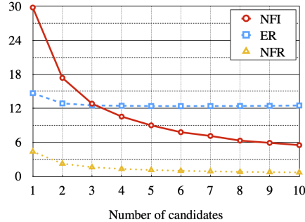
Figure 2: Effect of increasing number of candidates to NFI ( \downarrow ), NFR ( \downarrow ), and error rate (ER) ( s2s\text{-base} \Rightarrow s2s\text{-large} ).
