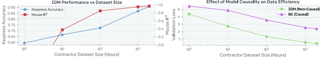
Figure 3: (Left) IDM keypress accuracy and mouse movement R^2 (explained variance 62 ) as a function of dataset size. (Right) IDM vs. behavioral cloning data efficiency.
