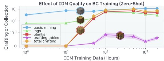
Figure 9: Zero-shot performance of BC models trained from scratch on the earlygame_keyword dataset labeled with IDMs that were trained on increasing amounts of contractor data.
