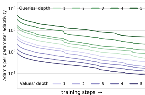
Figure 6: Adaptive learning rates computed by Adam in Transformers.
