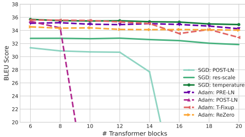
Figure 5: BLEU scores by increasing the number of transformers blocks. ‘X’ Transformer blocks implies in total ‘X’ encoder self-attention, ‘X’ decoder self-attention and ‘X’ decoder cross-attention layers.
