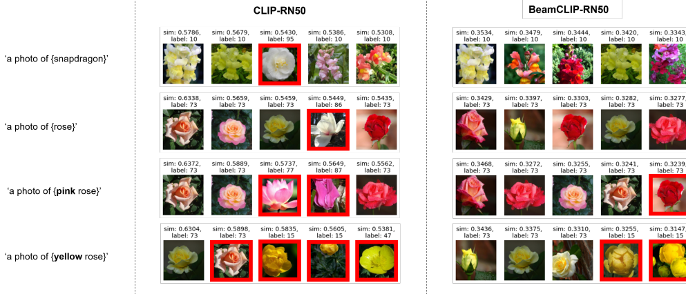
Figure 3: Comparison of CLIP-RN50 and BeamCLIP-RN50. This figure shows the top-5 text-image retrieval results. A red rectangle denotes an incorrect result. CLIP-RN50 provides many incorrect results, since its zero-shot accuracy is relatively low. In contrast, BeamCLIP-RN50 provides much improved results, since it is transferred from CLIP-ViT/16 with higher zero-shot accuracy.
