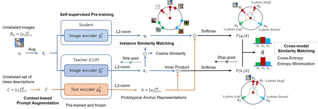
Figure 2: Overview of the BeamCLIP. Representation transfer can be viewed as a task in which, given a query input, a student model learns to regress a vector representation of a teacher model. The BeamCLIP first measures the normalized cross-modal similarity of the query image compared to anchor text representations in the teacher’s embedding space. Then, it encourages the student to mimic the same cross-modal similarity in the student’s embedding space. To better align image representations, our method uses self-supervised pre-training of the student model. Finally, to avoid text ambiguity, we use context-based prompt augmentation.
