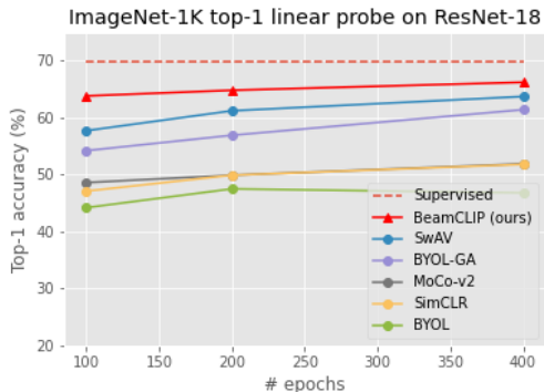
Figure 1: ImageNet-1K top-1 linear probe accuracy on ResNet-18 representations. By transferring CLIP-ViT [32] vision-language representations to ResNet-18, the BeamCLIP can learn better visual representations than vision-only self-supervised learning (SSL) methods in terms of the linear probe accuracy.
