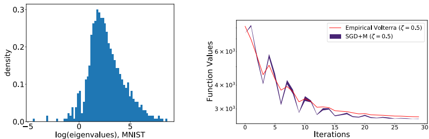
Figure 3: SGD+M vs. Theory on even/odd MNIST. MNIST ( 60,000 \times 28 \times 28 images) [16] is reshaped into a single matrix of dimension 60,000 \times 784 (preconditioned to have centered rows of norm-1), representing 60,000 samples of 10 digits. The target \mathbf{b} satisfies b_i = 0.5 if the i^{\text{th}} sample is an odd digit and b_i = -0.5 otherwise. SGD+M was run 10 times with (\Delta = 0.8, \gamma = 0.001, \zeta = 0.5) and the empirical Volterra was run once with (R = 11,000, \tilde{R} = 5300) . The 10^{\text{th}} to 90^{\text{th}} percentile interval is displayed for the loss values of 10 runs of SGD+M. While MNIST data set does not satisfy our eigenvalue assumption on the data matrix, the solution to the Volterra equation on MNIST data set captures the dynamics of SGD+M. See App. D for more details.
