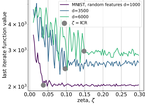
Figure 5: For each value of the batch fraction, \zeta , we run SGD+M for 50 iterations on (normalized) MNIST data set using a random features set-up with Gaussian weight matrix \mathbf{W} \in \mathbb{R}^{784 \times d} (see App. D for details) and targets odd/even. We record the function value of the last iterate. The momentum and learning rate parameters are set to be near-optimal (22). Gray dot is the computed ICR value. At the predicted \zeta = \text{ICR} (gray dot), there is a change in the behavior of the last iterate. For \zeta \leq \text{ICR} , the value of the last iterate monotonically decreases until it hits the ICR. For \zeta \geq \text{ICR} , we see no improvement in the value of the last iterate. This agrees with the theory that the convergence rate does not change.
