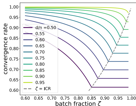
Figure 2: Convergence rate as batch size changes on a Gaussian random least squares problem with ratio r \stackrel{\text{def}}{=} \frac{d}{n} varying. Here \kappa = (1 + \sqrt{\frac{1}{r}})^2 / (1 - \sqrt{\frac{1}{r}})^2 and \bar{\kappa} = 1 / (1 - \sqrt{\frac{1}{r}})^2 . When \zeta goes above a specific value (see Proposition 5), the convergence rate freezes at 1/\sqrt{\kappa} . Otherwise the rate behaves like C/\kappa with a constant C = \zeta / (1 - \zeta) and we get no speed up from SGD+M.
