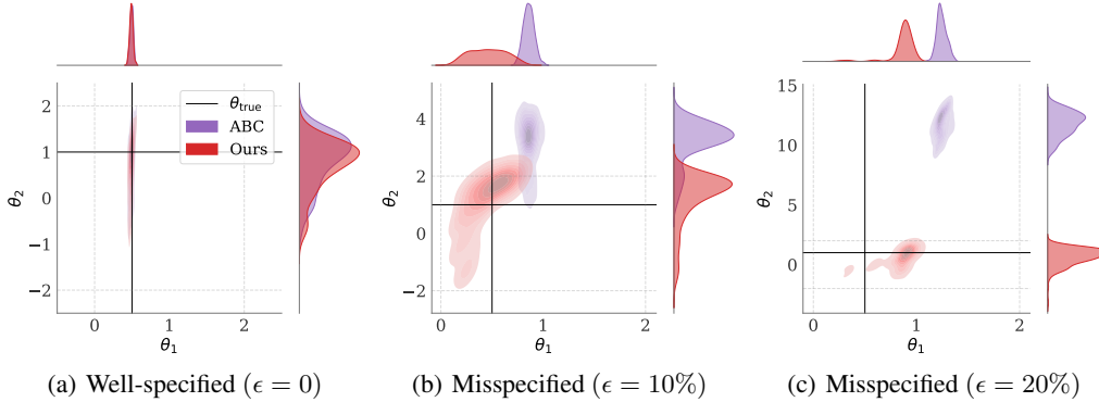
Figure 10: Ornstein-Uhlenbeck process. Posteriors obtained from our method (ABC-RS) and ABC for different degrees of model misspecification.
