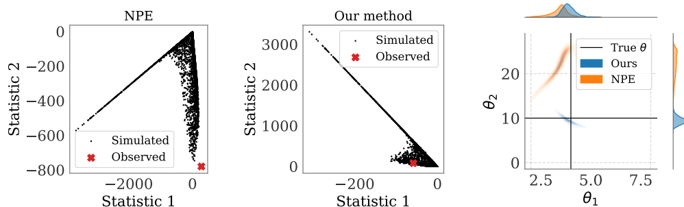
Figure 1: Inference on misspecified Ricker model with two parameters, see Section 4 for details. Left : Learned statistics obtained using NPE; each point (in black) corresponds to a parameter value sampled from the prior. The observed statistic (in red) is outside the set of statistics the model can simulate. Middle : Statistics learned using our robust method; the observed statistic is inside the distribution of simulated statistics. Right : The resulting posteriors obtained from NPE and our method. The posterior obtained from our method is close to the true parameter value, while that from NPE is completely off, going outside the prior range (denoted by dashed grey lines).
