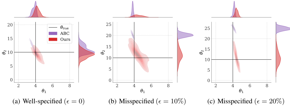
Figure 9: Ricker model. Posteriors obtained from our method (ABC-RS) and ABC for different degrees of model misspecification.
