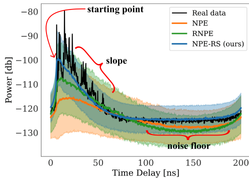
Figure 6: Predictive performance of NPE, RNPE and our NPE-RS method on the Turin model under misspecification. NPE-RS leads to the best fit. The shaded regions denote \pm 1 std. deviation of the posterior predictive distribution of each method.
