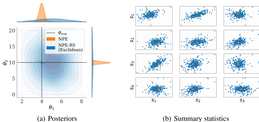
Figure 11: Ricker model . Posteriors and summary statistics for \mathcal{D} being the Euclidean distance.
