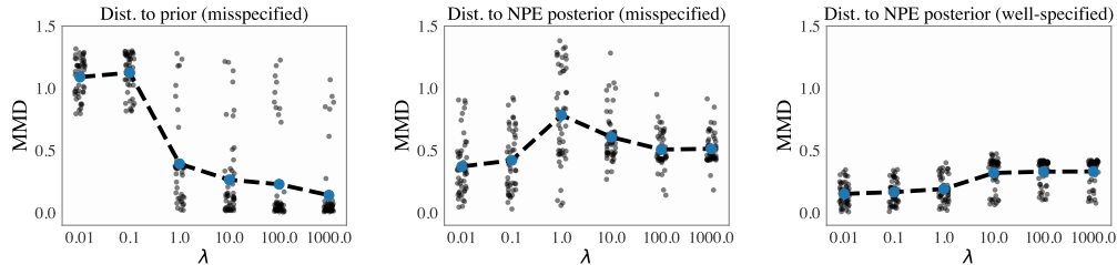
Figure 5: MMD between the NPE-RS posteriors and ( left ) the prior in the misspecified setting, ( middle ) the NPE posteriors in the misspecified setting, ( right ) the NPE posteriors in the well-specified setting, for different values of \lambda .
