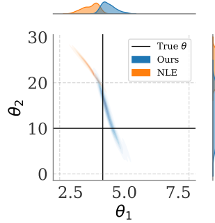
Figure 12: Ricker model. Posteriors obtained from our method (NLE-RS) and NLE. We set \epsilon = 10\% for this experiment.
