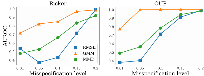
Figure 7: Misspecification detection experiment. AUROC of the proposed detection methods (GMM and MMD) versus misspecification level for the Ricker model and the OUP. The RMSE-based baseline is shown in blue.
