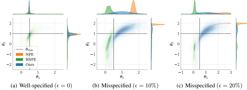
Figure 8: Ornstein-Uhlenbeck process. Posteriors obtained from our method (NPE-RS), RNPE, and NPE for different degrees of model misspecification.
