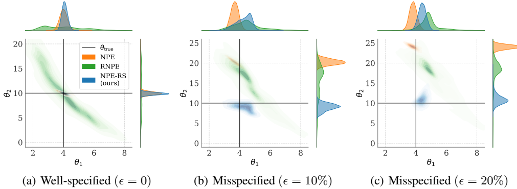
Figure 3: Posteriors obtained from NPE, RNPE, and our NPE-RS method for the Ricker model. We perform similar to NPE in the well-specified case, unlike RNPE. Under misspecification, NPE and RNPE posteriors drift away from \theta_{\text{true}} , going even beyond the prior range (denoted by dashed gray lines) in the case of NPE. Our method is robust to model misspecification.
