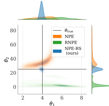
Figure 4: Posteriors from NPE, RNPE, and NPE-RS for Ricker model. NPE-RS is robust to prior misspecification.
