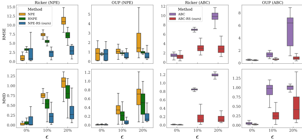
Figure 2: Performance of the SBI methods in terms of RMSE and MMD for both the Ricker model and OUP. Each box represents the median and interquartile range (IQR), while the whiskers extend to the furthest points within 1.5 times the IQR from the edges of the box. For the well-specified case ( \epsilon = 0\% ), the proposed NPE-RS and ABC-RS methods perform similar to their counterpart NPE and ABC, respectively. Under misspecification ( \epsilon > 0\% ), NPE-RS and ABC-RS achieve lower RMSE and MMD values, demonstrating robustness to model misspecification.
