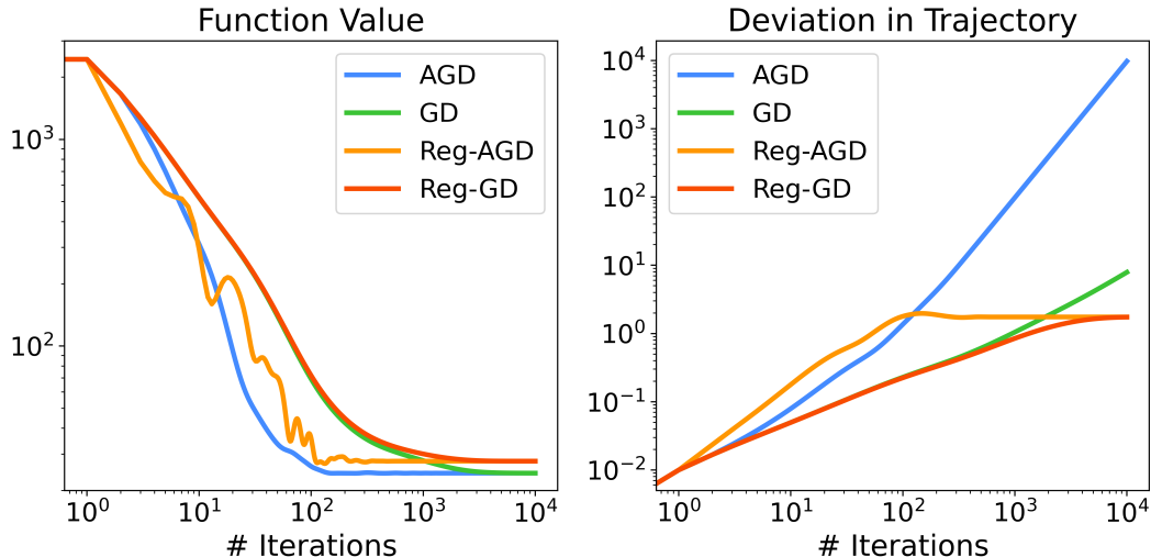
Figure 1: Comparisons among GD, AGD, and their regularized version on the quadratic minimization problem with \delta -inexact gradients. The left figure plots the convergence behavior and the right shows the reproducibility. Both axes are plotted utilizing a logarithmic scale.
