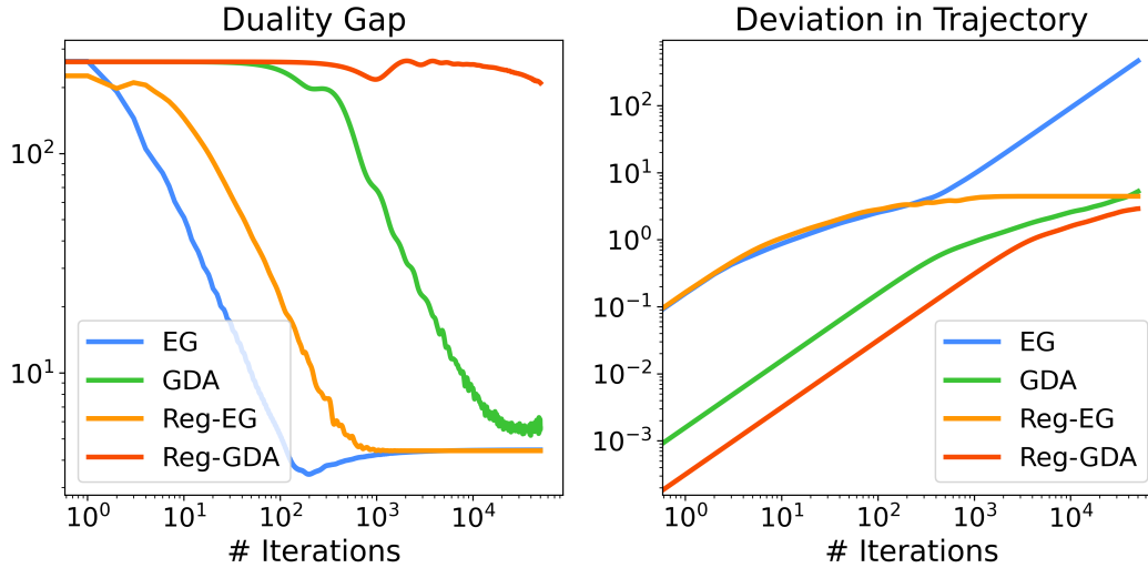
Figure 2: Comparisons among GDA, EG, and their regularized version on the bilinear matrix game with \delta -inexact gradients. The left figure plots the convergence behavior and the right shows the reproducibility. Both axes are plotted utilizing a logarithmic scale.
