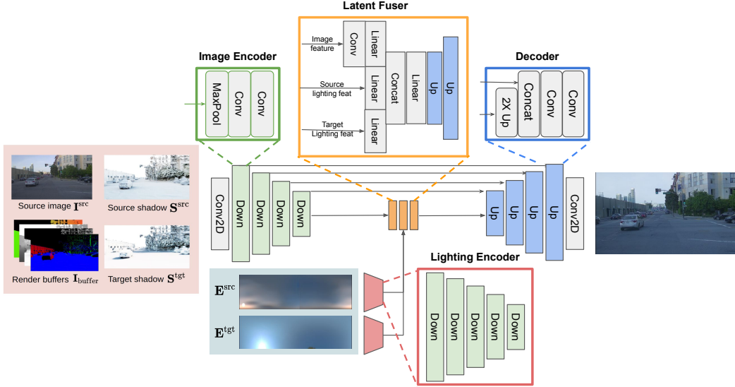
Figure A11: Network architecture of the neural deferred rendering module. Green, red, orange, and blue boxes denote the image encoder , lighting encoder , latent fuser and rendering decoder , respectively.
