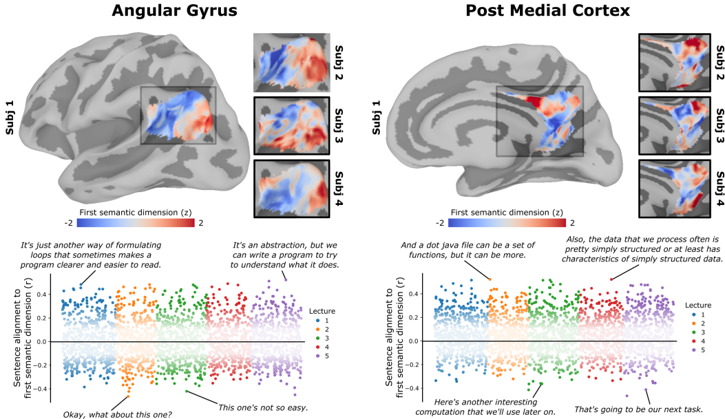
Figure 5: Learned projection of voxels and stimulus features, for the first semantic dimension. Fitting the H-HMM to the entire fMRI dataset produced projection matrices W_i for each subject and for the stimulus embedding. The voxel patterns (for the first four subjects) and sentences associated with the maximally-informative learned semantic dimension are visualized for both the angular gyrus (left) and posterior medial cortex (right). The voxel maps are broadly similar across subjects, but have distinct fine-scale structures specific to each individual. The scatter plots show the association between each sentence and the first semantic dimension across the 2,445 sentences in the dataset, highlighting example sentences that are strongly correlated or anti-correlated with this dimension.
