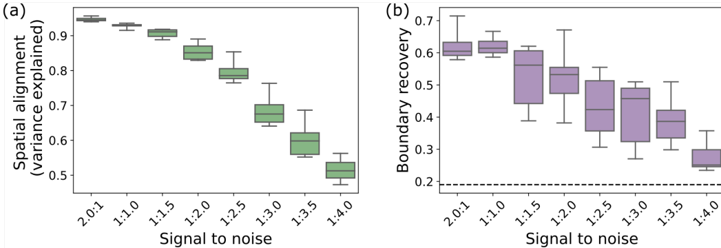
Figure 3: Model validation in simulated data. a) The model exhibits high alignment in the latent projections of held-out fMRI events (i.e. high variance explained by the event clustering) until the noise amplitude is several times larger than the simulated signal. b) The model can successfully recover ground-truth event boundaries for each subject up to high noise levels; the dotted line indicates the performance of a null model that randomly selects timepoints as event boundaries.
