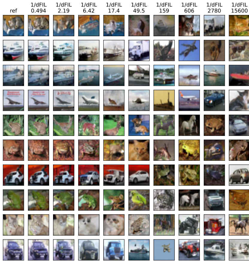
Figure 7: Results from DDPM [30]-based reconstruction attack. High 1/dFIL prevents exact pixel-to-pixel reconstruction, but images that share some high-level features with the original image can be generated unless 1/dFIL is not too high.
