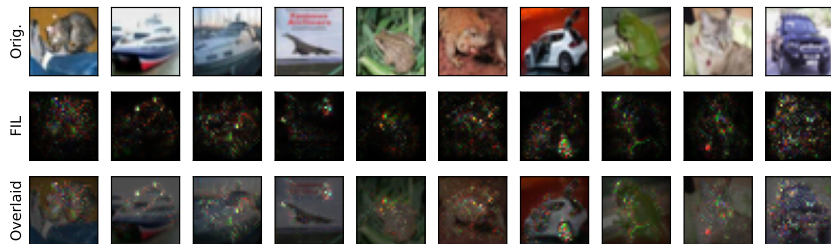
Figure 8: Per-pixel FIL from the ResNet-18 + CIFAR-10 split-middle setup in Section 4.2.2. Image best viewed with colors.
