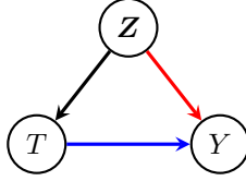
Figure 5: A generalised example of a static causal treatment model. The past P(T, \mathbf{Z}) (black) can be freely specified separately from the causal effect (blue). However, the dependency measure between \mathbf{Z} and Y (red), \phi should be parameterised in such a way that the margins P(\mathbf{Z}) and P(Y | \text{do}(T)) are invariant to changes in \phi .
