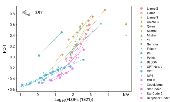
Figure B.1: PC-1 provides a smooth capability measure with a wider dynamic range than specific benchmarks like MMLU (Fig. E.4). In contrast to compute scale measures, it also enables the comparison of models from heterogeneous sources on a unified scale.
