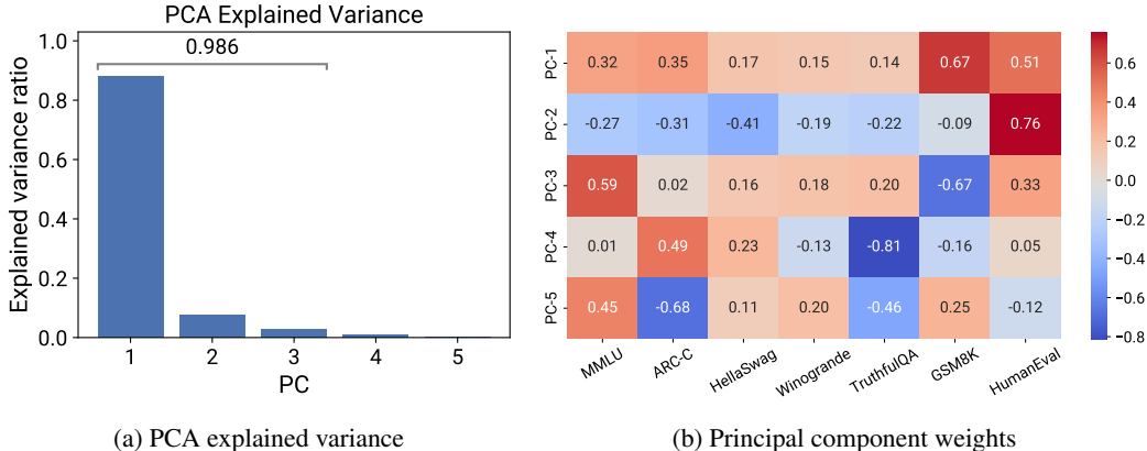
Figure E.1: The extracted PC measures for instruction-tuned LMs follow similar low-rank structures and interpretable patterns as pretrained base LMs (see Fig. 2).
