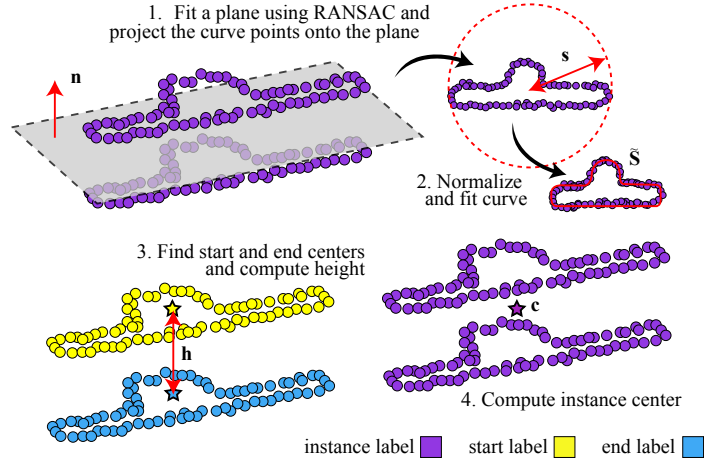
Figure 4: Converting 3D reconstructed geometry and semantics into CAD parameters.
