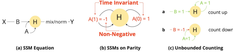
Figure 2: (a) Visualizing the SSM equations 1, 2: The hidden state H is updated by a combination of its previous values, transformed by matrix A , and the input X , modulated by matrix B . The updated hidden state and input are then processed through a Mix(\cdot) layer, which can incorporate components like (Swi)GLU or Linear layers, with an optional RMSNorm for normalization. (b) An intuitive construction for recognizing PARITY with SSMs is achieved by setting B = 0 and A = -1 when the input is 1, and A = 1 otherwise. However, this construction violates both NONNEGATIVE and TIME-INVARIANT properties. We show that one of these properties is provably required to recognize PARITY at arbitrary lengths using an SSM (Theorem 2). (c) Modeling a^n b^n : the matrix A adds the previous hidden state to the update, and depending on whether the input symbol requires counting up or down, matrix B is set to 1 or -1 , thus making the SSM simulate a counter (Theorem 5)
