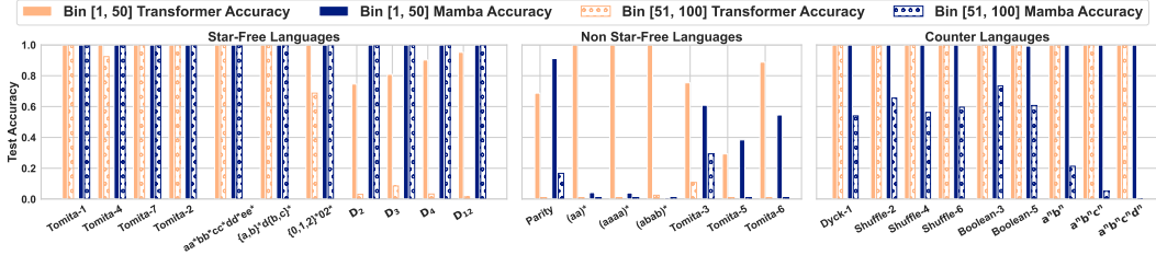
Figure 5: Results on 27 formal languages, comparing our Mamba results (blue) with transformer results reported by Bhattamishra et al. [2020] (orange), on in-distribution lengths (solid) and out-of-distribution lengths (dotted). As predicted by Theorem 4, Mamba performs strongly on star-free languages, and even shows perfect length generalization. Again as predicted by Theorem 4, it performs poorly on non-star-free languages. Results for transformers from Bhattamishra et al. [2020] are mixed. Mamba also succeeds on learning the counter languages from Theorem 5, showing perfect accuracy at in-distribution lengths at in-distribution lengths, but length generalization lags behind transformers.
