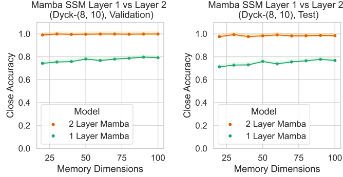
Figure 7: Mamba Accuracy on Dyck_{8,10} , on the development set (length \leq 700 , same length range as training set) and test set (length 700 \leq n \leq 1400 ). The latter is also plotted in Figure 4.
