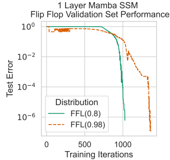
Figure 6: Test error on the validation set for \mathcal{L}_{FF} , following Liu et al. [2023a]. Mamba shows near-zero test error in both In- (green) and Out-of-distribution (orange) settings, consistent with Theorem 1, and avoids the failure seen in transformers [Liu et al., 2023a]
