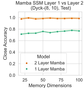
Figure 4: As predicted by Theorem 6, Mamba with 2 layers can model Dyck(K, h) . Results for test set with strings of length 700 \leq n \leq 1400 .
