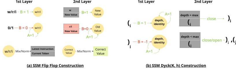
Figure 3: (a) Construction for Flip-Flop (Theorem 1): The first layer stores instruction bits to the hidden state, while data bits are forwarded to the output. Hence, the output always contains both the latest instruction and the associated data bit. In the second layer, if the instruction bit is w , the corresponding data bit is written to the hidden state, else the old value persists. This allows the model to consistently output the correct data bit. (b) Construction for Dyck( K, h ) (Theorem 6): The first layer tracks the depth by counting up for each opening bracket, and down for each closing bracket. The second layer builds on the Flip-Flop construction to find the last opening bracket at the current depth; the next symbol can be either the matching closing bracket or – if the maximum depth has not been reached – an arbitrary opening bracket.
