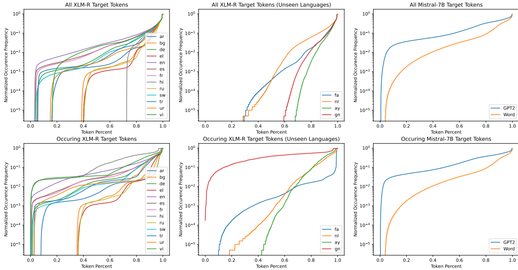
Figure 6: Analyzing how often the hypernetwork sees the tokens of different target tokenizers during training. Note the logarithmic y-scale. We analyze the occurrence for all tokens in the target vocabulary (top) and for tokens which occur at least once in the evaluation data (bottom) across target tokenizers in seen languages for XLM-R (left), unseen XLM-R languages (middle) and English Mistral-7B tokenizers (right). The bottom row is more informative w.r.t. how well the hypernetwork generalizes to unseen tokens since tokens which do not occur do not substantially impact evaluation.
