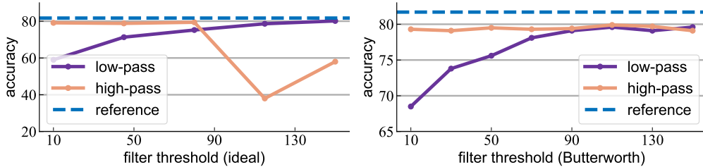
Figure 26: Accuracy on filtered images at different thresholds. For most thresholds, both ideal and Butterworth filters achieve high accuracies for both high-pass and low-pass filters.
