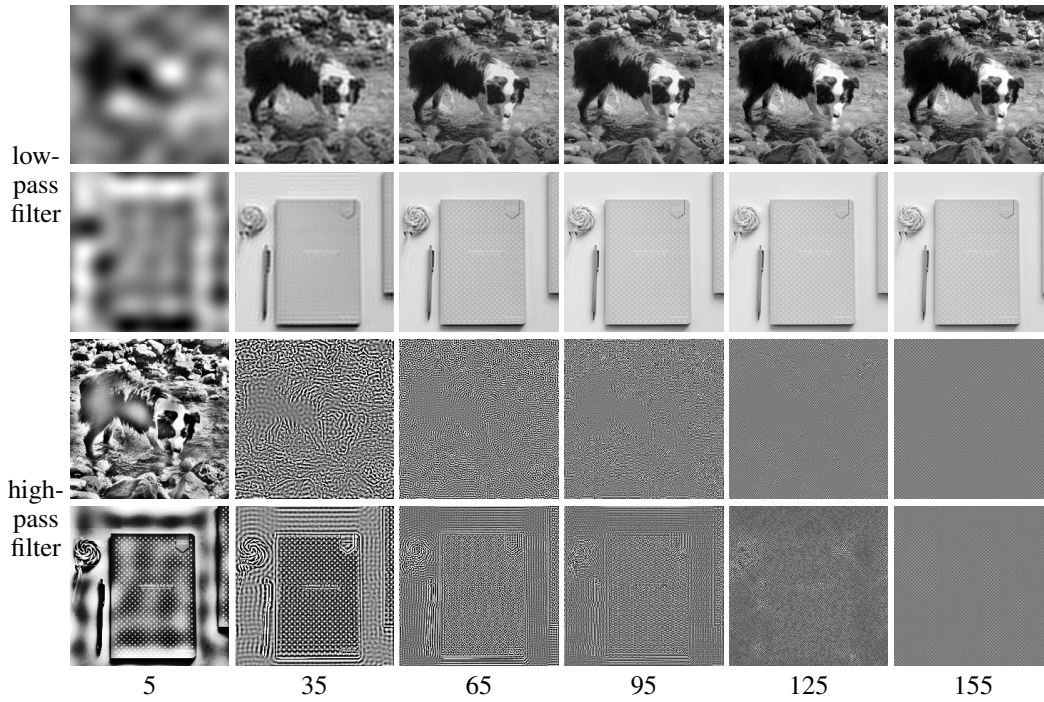
Figure 24: Ideal filter [22] with different thresholds. We select filtering thresholds {5, 35, 65, 95, 125, 155}. The high-pass filtered images are equalized for better visualization.
