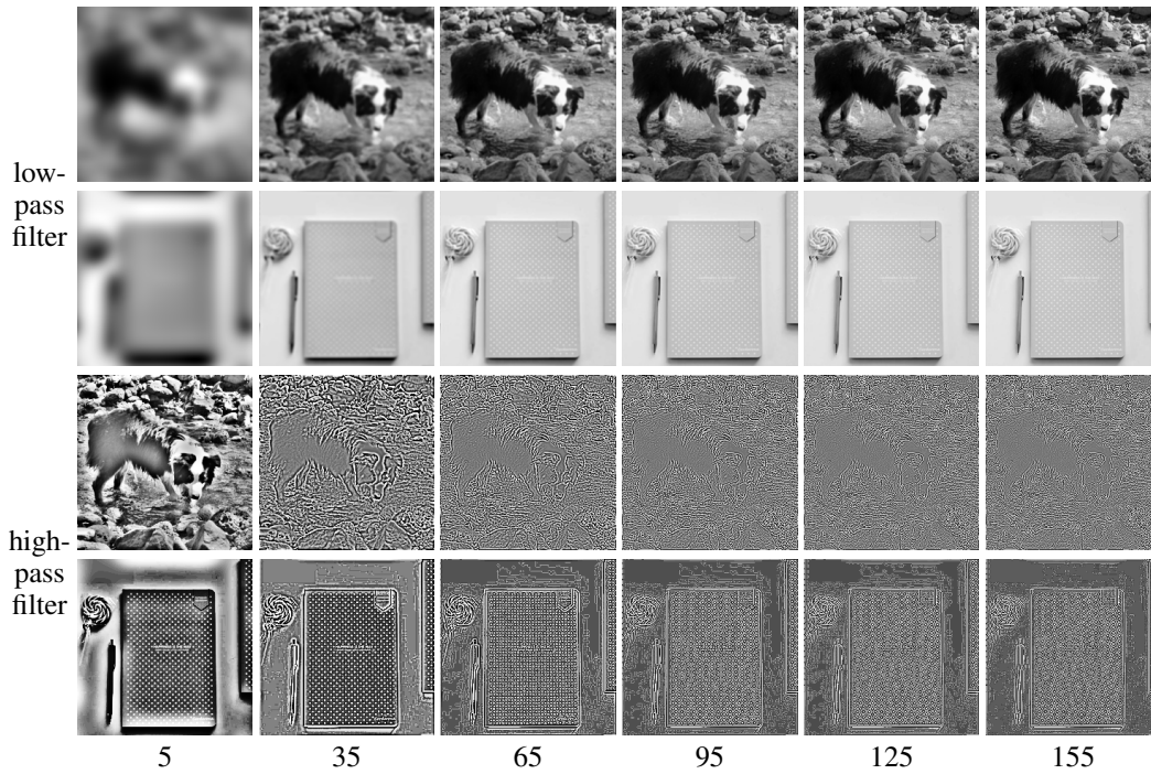
Figure 25: Butterworth filter [9] with different thresholds. We select filtering thresholds {5, 35, 65, 95, 125, 155}. The high-pass filtered images are equalized for better visualization.
