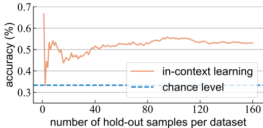
Figure 18: The accuracy of in-context learning converges at 160 samples per dataset.
