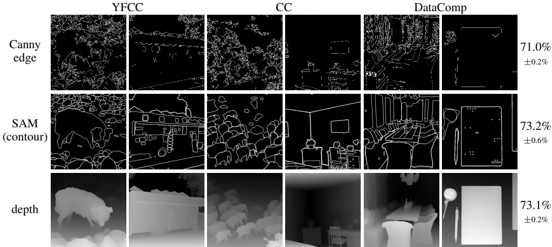
Figure 3: Transformations outlining object shapes and estimating pixel depth. Dataset classification achieves even higher accuracies on object contours and depth images than on semantic information, indicating that object shapes and spatial geometry vary significantly across YCD.
