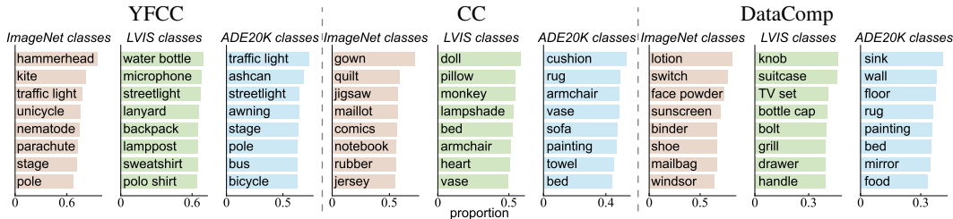
Figure 11: Object classes with the highest proportions of YFCC, CC, or DataComp images. Less-frequent classes are not shown. Most classes consist predominantly of images from one dataset.
