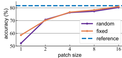
Figure 5: Effect of patch sizes. Dataset classification accuracy approaches the reference one with larger patch sizes.
