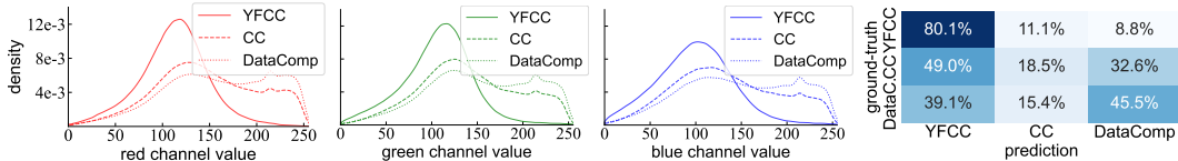
Figure 7: Distribution of mean RGB values and confusion matrix. YFCC’s RGB values are overall smaller, while CC’s and DataComp’s are very similar. This is also reflected in the confusion matrix of dataset classification on mean RGB images, where YFCC can be classified very easily (indicated by the dark blue box on the top left), while there is high confusion between CC and DataComp.
