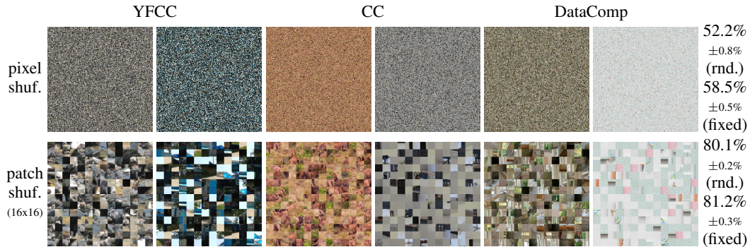
Figure 4: Transformations breaking spatial structure. Pixel shuffling drastically decreases dataset classification accuracy, but patch shuffling has minimal impact. This demonstrates that local structure is important and sufficient for models to learn the patterns of each dataset.
