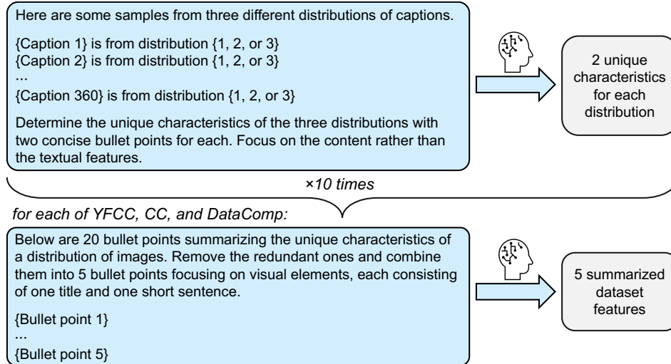
Figure 19: Prompting procedure for LLM summarization. The LLM summarizes the dataset characteristics over 10 iterations, with 360 randomly sampled captions per iteration. These characteristics are then aggregated, and the LLM consolidates them into five bullet points for each dataset.
