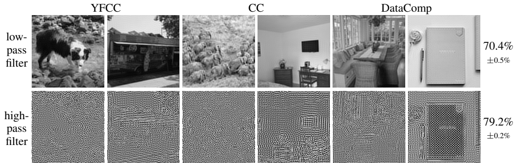
Figure 8: Transformations filtering high-frequency and low-frequency components retain close-to-reference accuracy. This indicates that dataset bias exists in different frequencies. The high-pass filtered images are equalized for better visualization.
