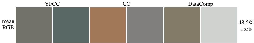
Figure 6: Averaging each color channel. Even when the values of each channel in images are averaged, the model can still achieve non-trivial dataset classification performance.
