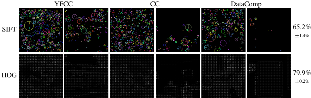
Figure 21: Transformations encoding handcrafted features. SIFT keypoints can moderately capture dataset bias, while HOG achieves close-to-reference accuracy by capturing local gradients.
