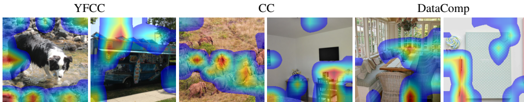
Figure 10: Grad-CAM heatmap [82, 61] on the dataset classification model trained on original datasets. The model focuses on specific objects to determine the dataset origin of each image.
