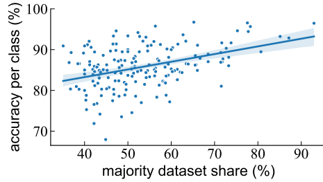
Figure 29: Majority dataset share for each ImageNet object class positively correlates with the reference dataset classification accuracy on YCD images within that object class.
