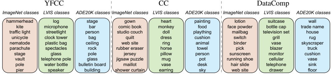
Figure 13: Object class ranking from logistic regression coefficients. The regression classifies images based on object presence. YFCC has more top objects related to outdoor scenes, while CC and DataComp focus on household items and products. Classes with low frequencies are not shown.
