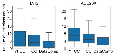
Figure 12: Unique object classes per image. On average, YFCC contains the highest number of unique objects in each image, followed by CC, while DataComp exhibits the lowest.
