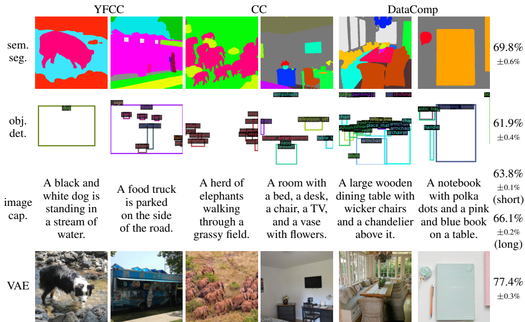
Figure 2: Transformations preserving semantic information (semantic segmentation, object detection, and caption) and potentially reducing low-level signatures (VAE) result in high dataset classification accuracy. This suggests that semantic discrepancy is an important form of dataset bias.
