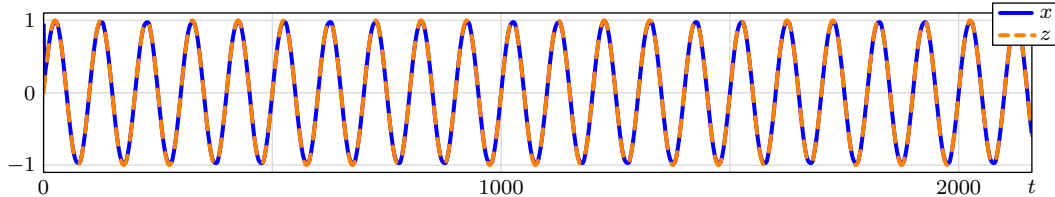
Figure 2: Recurrent net with 5 neurons, q = 1000 (accuracy term), r_w = 1 (weight regularization term), r = 0.1 (derivative of the weight term).
