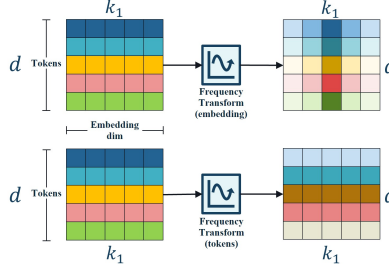
Figure E.1: Two directions of the proposed Frequency Transform. \text{FouRA}_{emb} computes the frequency transform along the embedding dimension (top), whereas \text{FouRA}_{token} computes the frequency transform across all the tokens (bottom).
