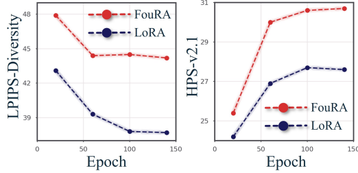
Figure E.3: Studying the training curves for signs of data-copying artifacts: We analyzed the effect of early stopping of training by measuring the performance. All results are with rank 64 and \alpha = 0.8 on the paintings adapter.
