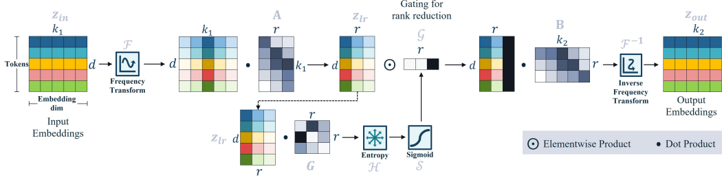
Figure 3: Operational diagram of FouRA. Illustrating the components of Eq. 5.
