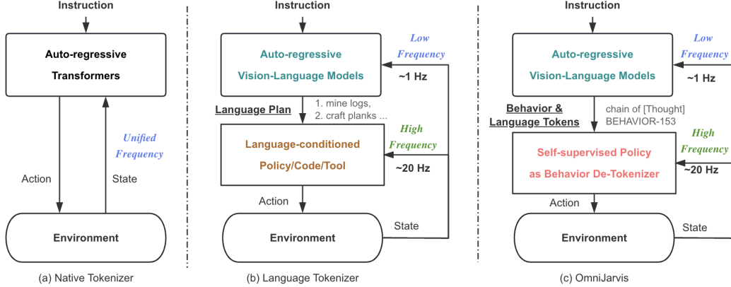
Figure 8: Comparative Framework of Vision-Language Action Models. (a) depicts a model where upon receiving a language instruction, actions are directly output based on the environmental state, facilitating immediate interaction with the environment at a unified frequency. Smaller models with <1B parameters like VPT [2] maintain higher frequencies (>20Hz), though their capability for complex reasoning tasks is limited. Larger models with >7B parameters such as RT-2 [6], offer enhanced performance but operate at significantly reduced frequencies (2-3Hz). (b) illustrates a common approach utilizing large vision-language models for planning, subsequently outputting language goals [46, 14, 4]. A language-conditioned policy then translates these language goals into actions at a real-time interaction rate of 20Hz, with high-level models re-planning at less than 1Hz. This hierarchical structure balances interaction frequency and performance, while it requires language as an intermediary and additional language labels. The training process of high-level vision-language models and language-conditioned policies are separate, thus performing poorly on tasks that can not be easily connected by language. (c) (ours) mirrors the hierarchical structure of (b) but differentiates by employing a self-supervised encoder-decoder policy [10] and FSQ quantization [34] as a behavior tokenizer. The upper-level vision-language models produce self-supervised behavior tokens, which are then conditioned by a policy decoder to output actions, facilitating environment interaction. The behavior tokens are injected into the training corpus of vision-language-action models, which enables end-to-end inference. This approach also eliminates the need for external language supervision and scales efficiently.
