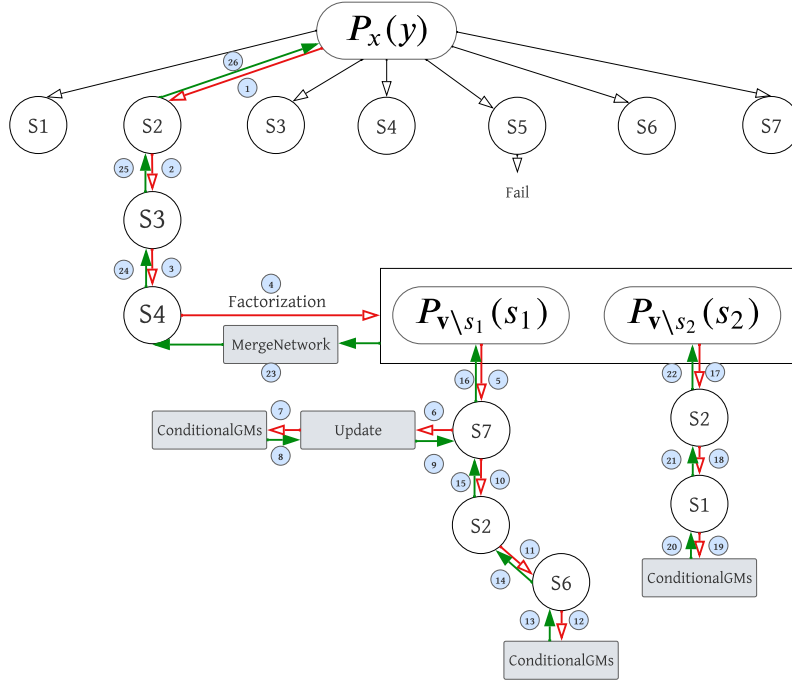
Figure 10: ID-GEN Recursion Tree Example
