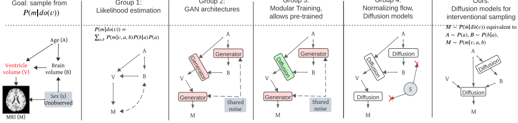
Figure 9: Suppose we aim to sample from P(m|\text{do}(v)) , with M (MRI) as high-dimensional. Group 1 includes algorithms (ex: ID) that depend on likelihood estimation such as P(m|v, a, b) . Group 2 algorithms with GAN architectures have issues with GAN convergence while Group 3 improves convergence with modularization but both struggle to match the joint distribution. Group 4 utilizes normalizing flow, diffusion models, etc but cannot deal with confounders. Groups 2-4 only do unconditional interventions or costly rejection sampling. Finally, our method can employ classifier-free diffusion models to sample from P(m|\text{do}(v)) or conditional P(m|a, \text{do}(v)) . The causal graph is adapted from Ribeiro et al. [41].
