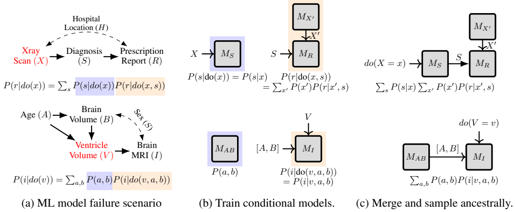
Figure 1: (Top: x-ray to report generation task) (a) do(X = x) removes the X \leftrightarrow R bias and makes the generation of R domain invariant. P(r|do(x)) is factorized into c-factors and (b) conditional models ( \{M_{V_k}\}_k ) are trained for each factor (shown as boxes). (c) The intervened value X = x is propagated through the merged network and samples from the P(r|do(x)) are generated.
