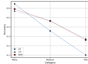
(b) Accuracy on ImageNet-LT with SAM
