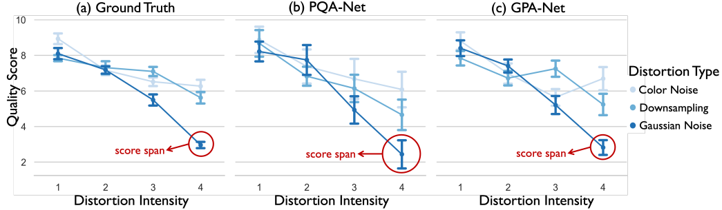
Figure 1: Statistics of SJTU-PCQA (part) [46] and predicted quality scores of NR-PCQA models (PQA-Net [21] and GPA-Net [32]). Quality scores of different distortion types are in lines of different colors. Red circles are to highlight the score span of different contents with the same distortion.
