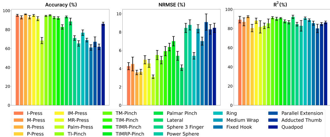
Figure 3: Quantitative evaluation of the user-independent model, showing the posture-wise performance on the estimation of hand pressure. The error bars indicate standard error.
