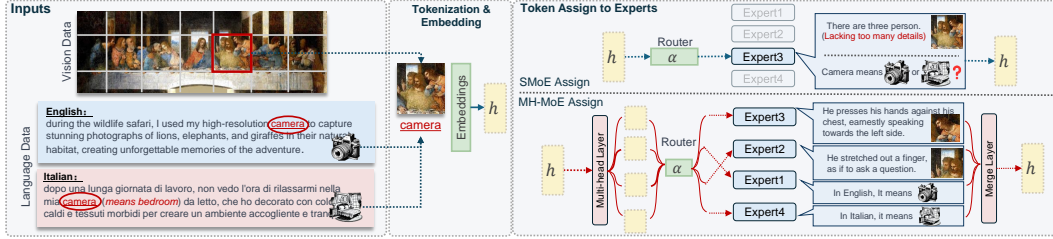
Figure 2: Workflow of MH-MoE. For vision data, different heads routed to different experts try to capture different aspects of details within patches and relations between patches. For language data, different heads attend to capture the varying contexts of false cognates across different languages (e.g., Italian and English) or polysemous words within a single language.
