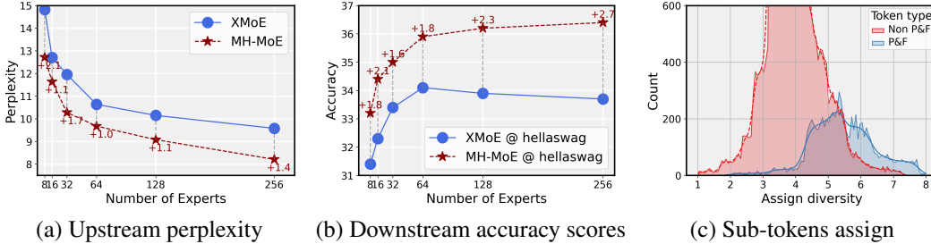
Figure 7: (a) Upstream training perplexity ( \downarrow ) when scaling the number of experts for both X-MoE and MH-MoE. (b) Accuracy scores on the hellaswag task when scaling the number of experts for both X-MoE and MH-MoE. (c) Comparison for sub-tokens assign diversity (the number of different experts they are routed to) for P&F and Non P&F tokens.
