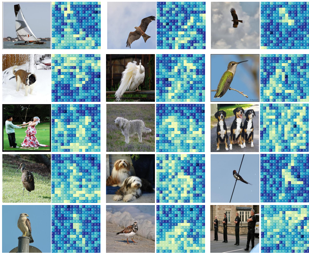
Figure 11: More visualization examples for assign diversity of sub-tokens split from different patches with respect to training steps. We analyze MH-MoE with 8 heads ( h=8 ) as the subject. Brighter regions indicate that sub-tokens from this patch are distributed to a greater number of diverse experts, while darker regions indicate that sub-tokens are assigned to more of the same experts.
