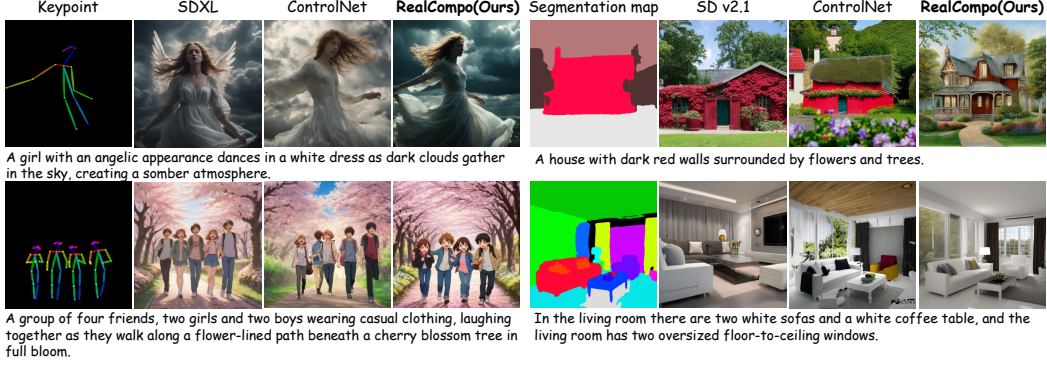
Figure 3: Extend RealCompo to keypoint- and segmentation-based image generation.
