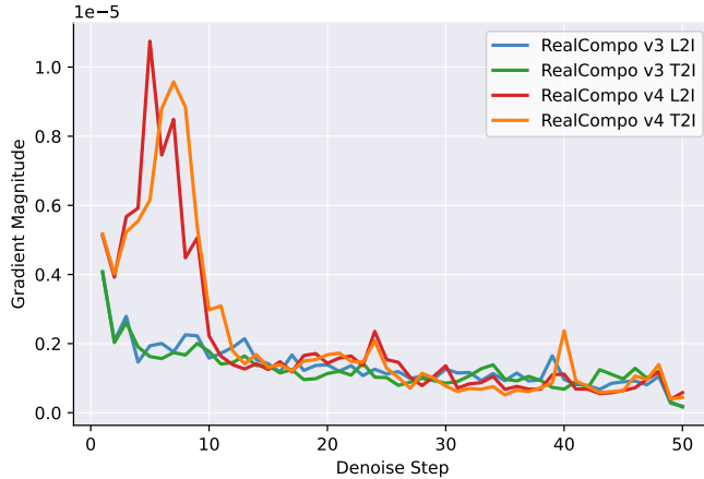
Figure 13: Changes of gradient magnitude in Eq. 7 across all denoising process for the T2I and L2I models of RealCompo v3 and v4.
