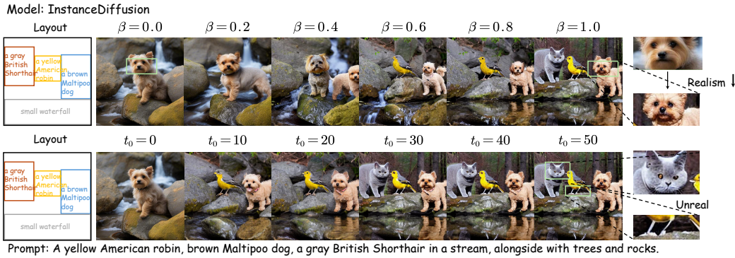
Figure 11: A more intuitive and clearer example to showcase our discoveries and motivation, using InstanceDiffusion [53].
