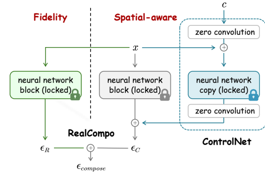
Figure 4: RealCompo constructed on ControlNet.
