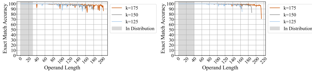
Figure 11: Left: Exact match accuracy of five models trained on size 30 data, offset randomization hyperparameter k = 125, 150 and 175 . Right: Exact match accuracy of five models trained on size 40 data, offset randomization hyperparameter k = 125, 150 and 175 .
