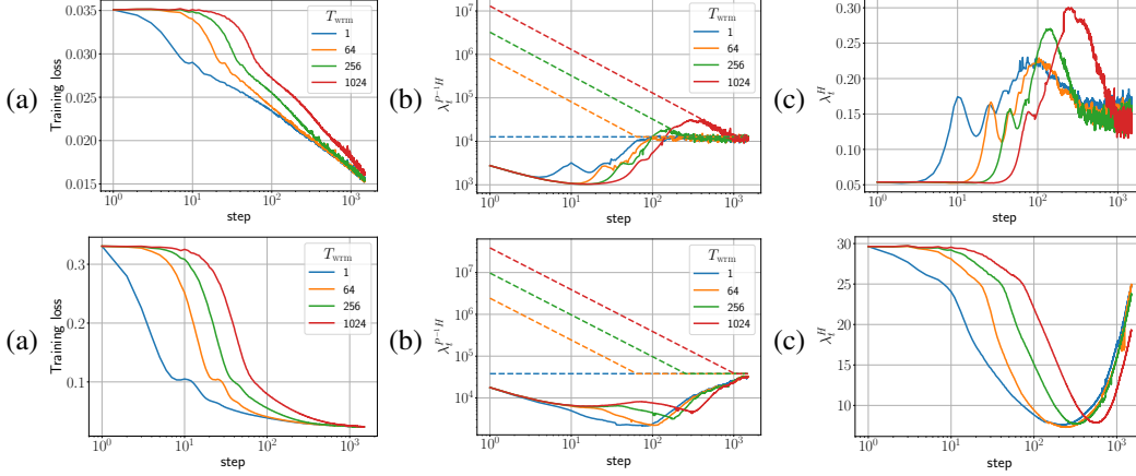
Figure 32: Training loss and sharpness trajectories of FCNs in (top) \mu\text{P} and (bottom) \text{SP} . The experimental setup is identical to Figure 2 but with GI-Adam instead of standard Adam.
