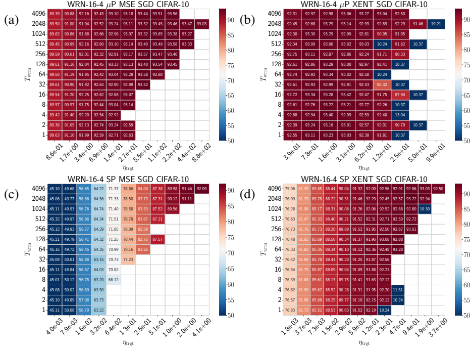
Figure 3: Test accuracy heatmaps of WRNs trained on CIFAR-10 using different and parameterizations loss functions using SGD: (a) \mu\text{P} and MSE loss, (b) \mu\text{P} and cross-entropy loss, (c) SP and MSE loss, and (d) SP and cross-entropy loss. Empty cells correspond to training divergences. Similar phase diagrams are generically observed for different architectures and datasets, as shown in Appendix F.
