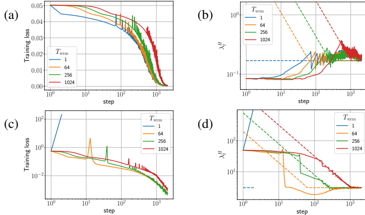
Figure 1: Training loss and sharpness trajectories of FCNs trained on a 5k subset of CIFAR-10 with MSE loss using GD. In the sharpness plot, the dashed lines represent the 2/\eta_t curves, and when \lambda_t^H is above these curves, training exceeds the instability threshold ( \eta > \eta_c ). (top) \mu\text{P} with \eta_{\text{tgt}} = 1/\lambda_0^H , (bottom) \text{SP} with \eta_{\text{tgt}} = 32/\lambda_0^H . Similar mechanisms are observed across different architectures, loss functions, and mini-batch sizes, as shown in Appendix E.
