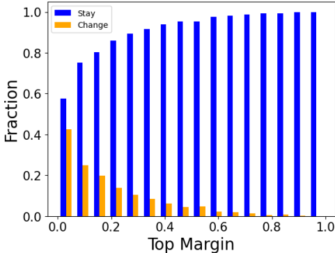
Figure 4: When the Top Margin is low, answer will more likely change (Llama2-70b, BnB W4A4, MMLU 5-shot)
