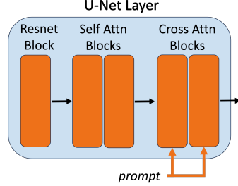
Fig. S 1: Single block of a U-Net layer (Stable Diffusion [31]).
