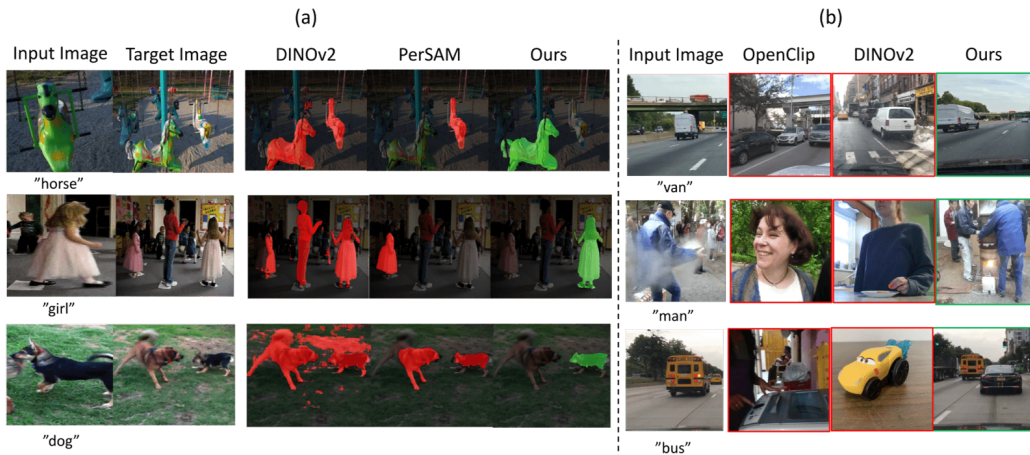
Figure 5: Qualitative Comparison: (a) Personalized Segmentation: Red and green indicate incorrect and correct segmentation, respectively. Our method accurately recognizes the reference instance despite significant variations (view angle, pose, or scale), while other methods often capture false positives from the same category. (b) Image Retrieval: Top-1 retrieved image is shown for each method. Note how our model identifies images containing the same instance, despite their small size and large variations. Other methods tend to capture only semantic similarity. Retrieval images have been zoomed in and cropped for clarity.
