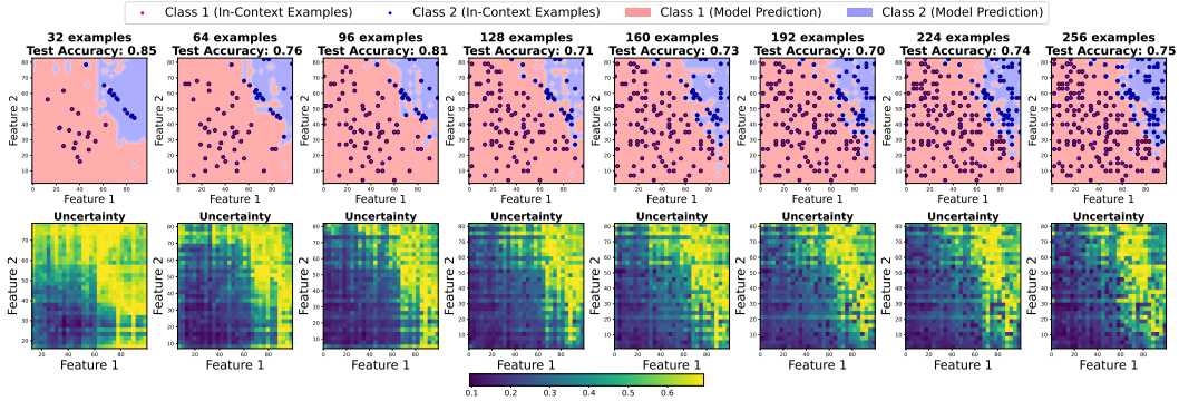
(b) Decision boundaries with different numbers of context examples when using random sampling.
