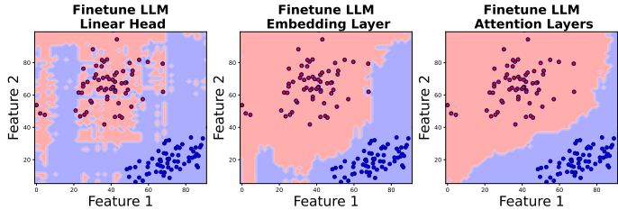
Figure 8: Decision boundary of Llama3-8B post finetuning the linear head, embedding layer and the attention layers. Finetuning the latter two layers improves the smoothness.
