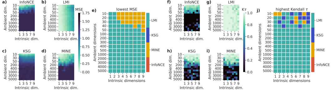
Figure 2: MI estimator performance scaling with increasing dimensionality. a) - d) Absolute accuracy measured by mean-squared error over 10 estimates per setting, with ground truth MI between 0 and 2 bits, and 2 \cdot 10^3 samples per estimate (1:1 training split for neural network-based estimators). e) Estimator with highest absolute accuracy in each setting. Ties broken randomly. f) - i) Relative accuracy measured by Kendall \tau rank correlation of estimates with ground truth. j) Estimator with highest relative accuracy in each setting. Ties broken randomly.
