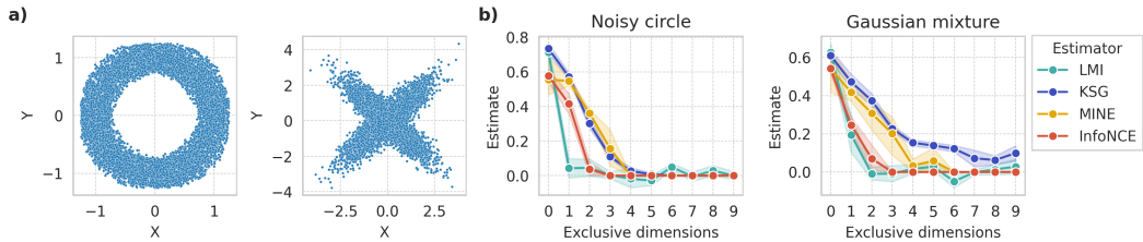
Figure 5: Constructing problems where LMI fails. a) Examples of symmetric distributions where \mathbb{E}[X|Y] = \mathbb{E}[X] . b) MI estimates from 10^3 samples of symmetric variables as exclusive (independent normal) dimensions are added. Ideal estimators are invariant. LMI latent space is 1D per variable.
