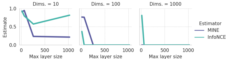
Figure 14: Variational bound estimators with increasing critic complexity, evaluated on multivariate Gaussians with 1-dimensional dependence structure. Each estimation problem has 5 \cdot 10^3 samples and ground truth MI of 1 bit.
