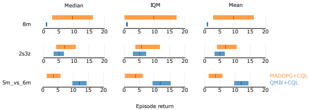
Figure 2: Comparing the performance of QMIX+CQL and MADDPG+CQL, two algorithms that could reasonably be called MACQL in the literature (see Table 1), using the Medium dataset from three different SMACv1 scenarios. We see that the difference in performance of these algorithms is significant, and depends on the scenario considered.
