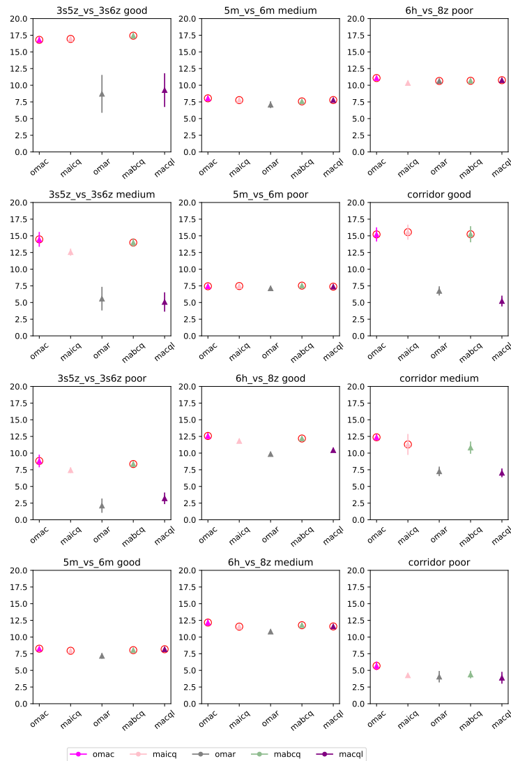
Figure 5: Results reported by Wang and Zhan (2023) on the SMAC environment.
